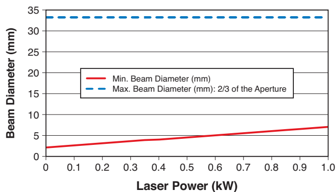
PM1K+ Beam Size 1,2 vs Power Plot
