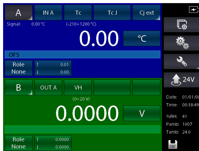
Figure 67 – Offset function activated
