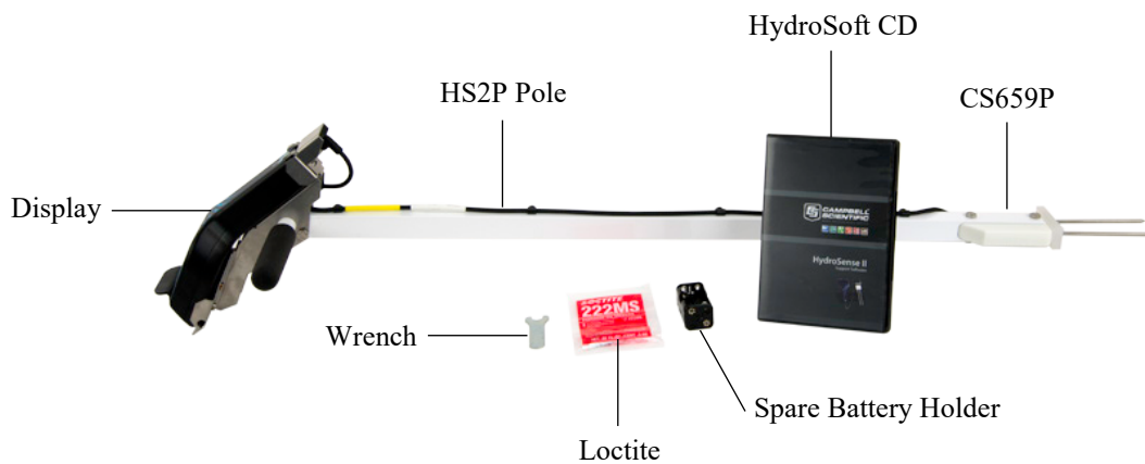
FIGURE 4-3. HS2P Parts
