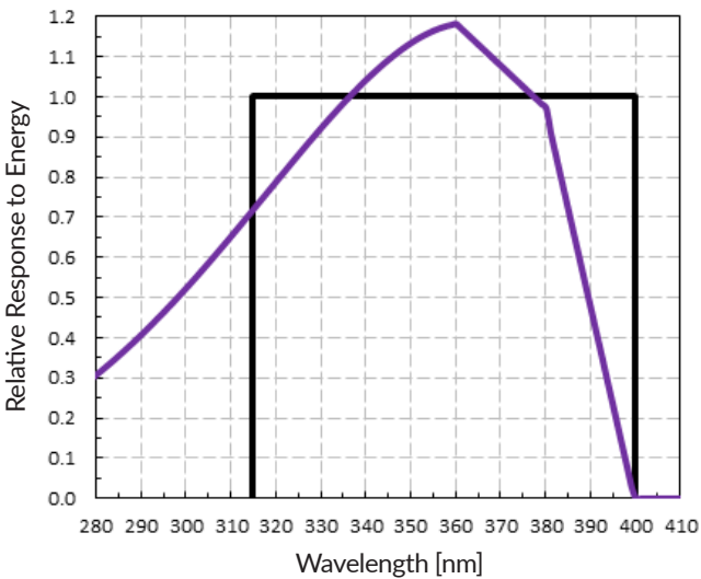
Spectral response estimate of Apogee SU-200 UV-A sensors. Spectral response was modeled from sensitivity of the photodetector and transmittance of the diffuser.
