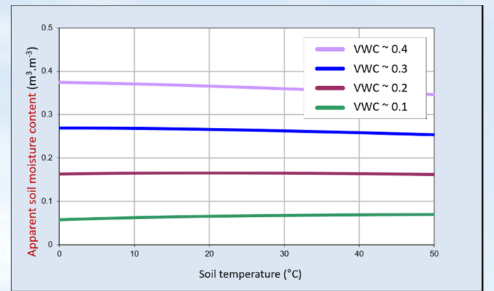
Temperature dependence of SM150T readings in a clay soil
