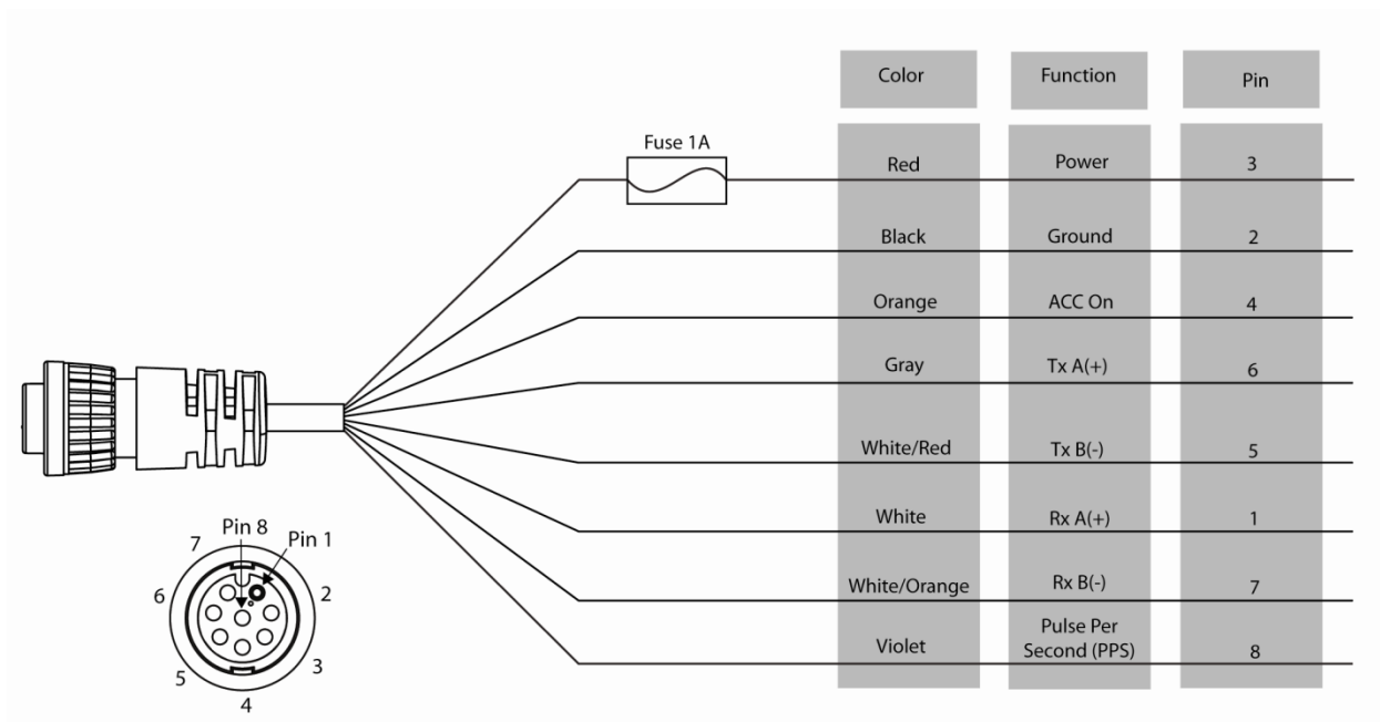
Figure 3b. GPS 19x NMEA 0183 HVS Power/Data Cable
