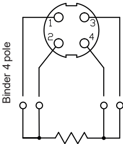
Connector pin-out
