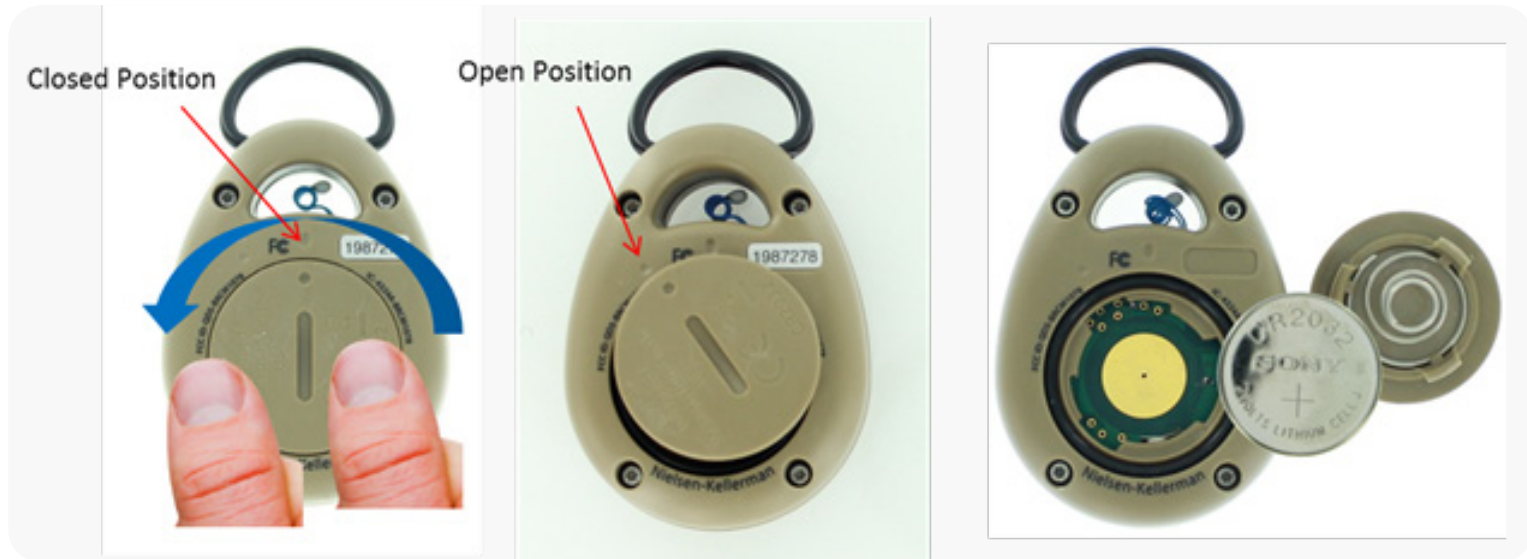
Figure 2: Battery Replacement
